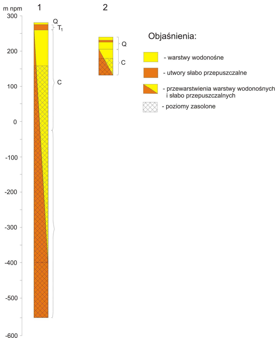
Rys. 4 Profile JCWPd 134
